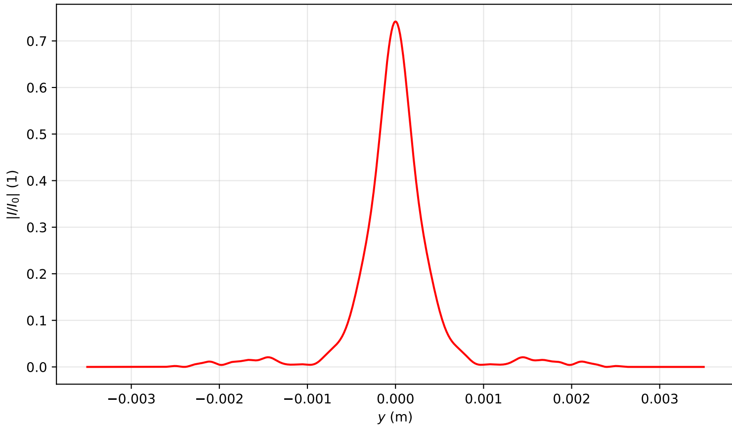
Intensity profile I(x=0, y, z=3.821)/I_0 , P_{in}=3.0P_{cr} , artificial time
